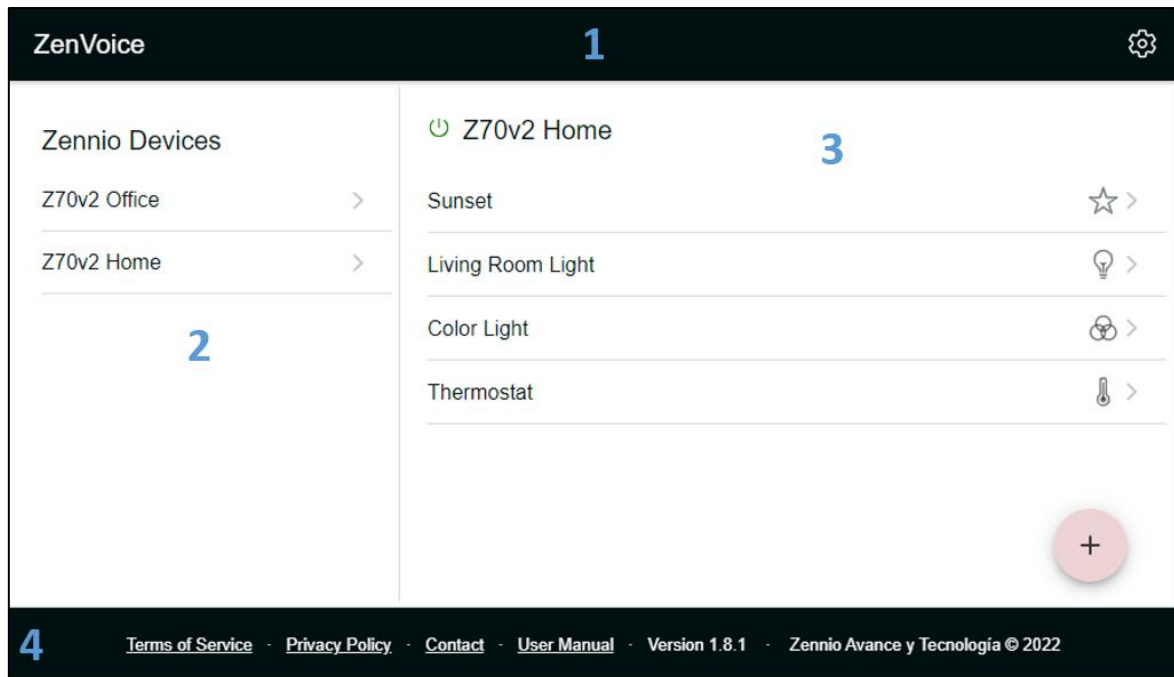
Figure 2. Main menu structure
