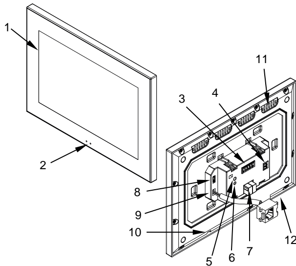
Figure 1 Schematic diagram (Z50)
