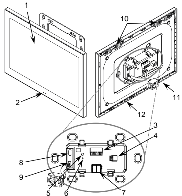
Figure 2 Schematic diagram (Z50)
