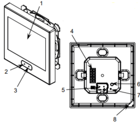
Figure 1. Schematic diagram.
