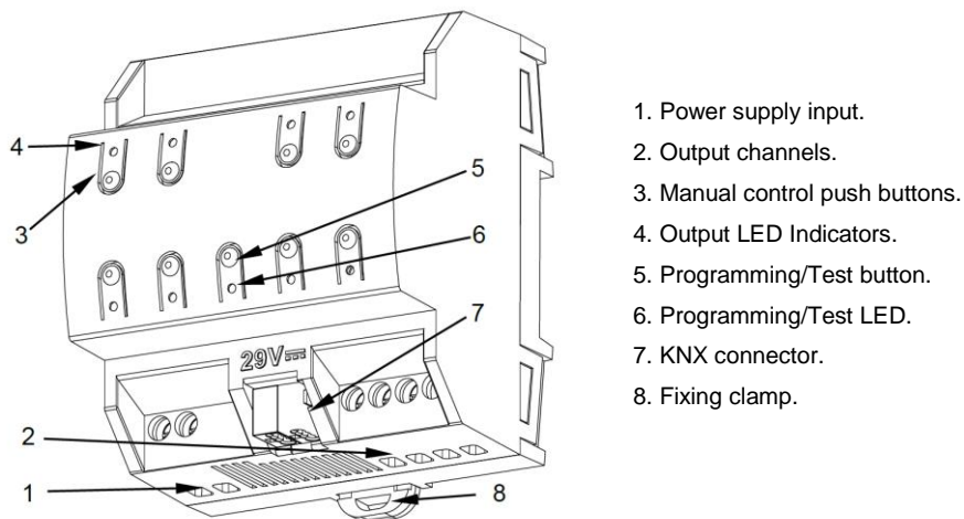
Figure 3 NarrowDIM X4 Element Diagram.
