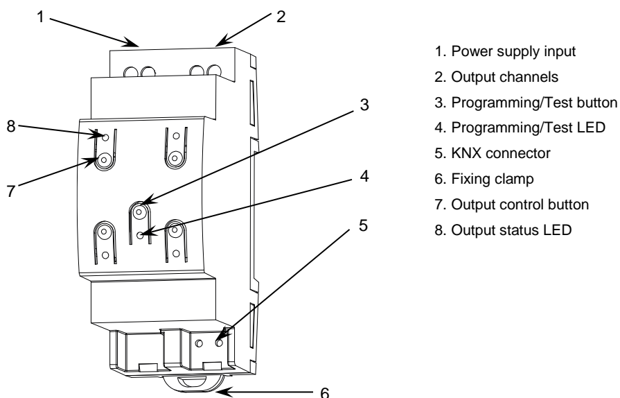
Figure 4 NarrowDIM X2 Element Diagram.
