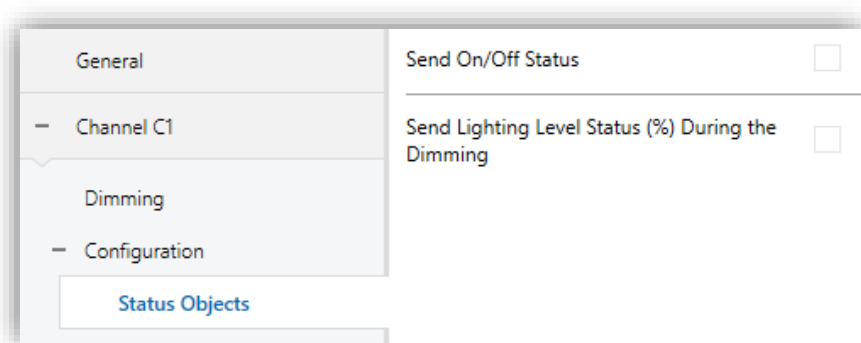
Figure 12 Status Objects.
