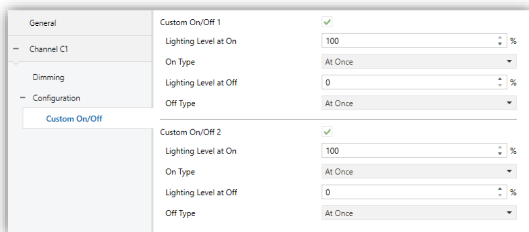
Figure 13 Custom On/Off.
