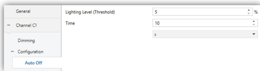
Figure 21 Auto Off.
