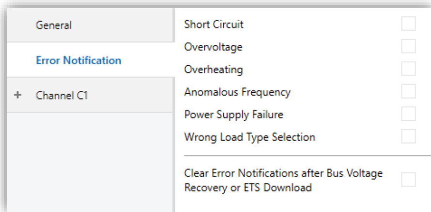
Figure 23 Error Notification.
