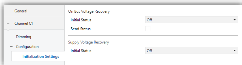
Figure 22 Initialization Settings.
