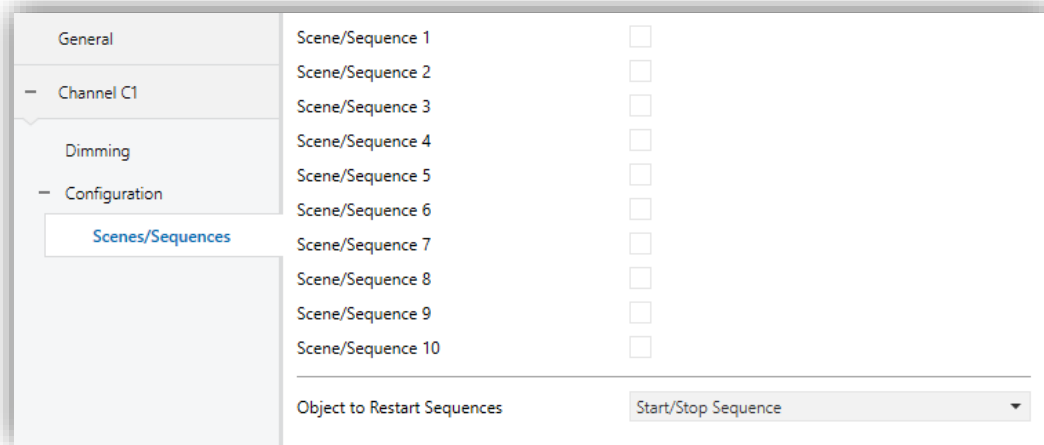
Figure 16 Scenes/Sequences.
