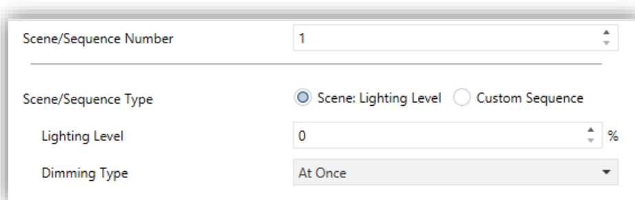
Figure 17 Scene.
