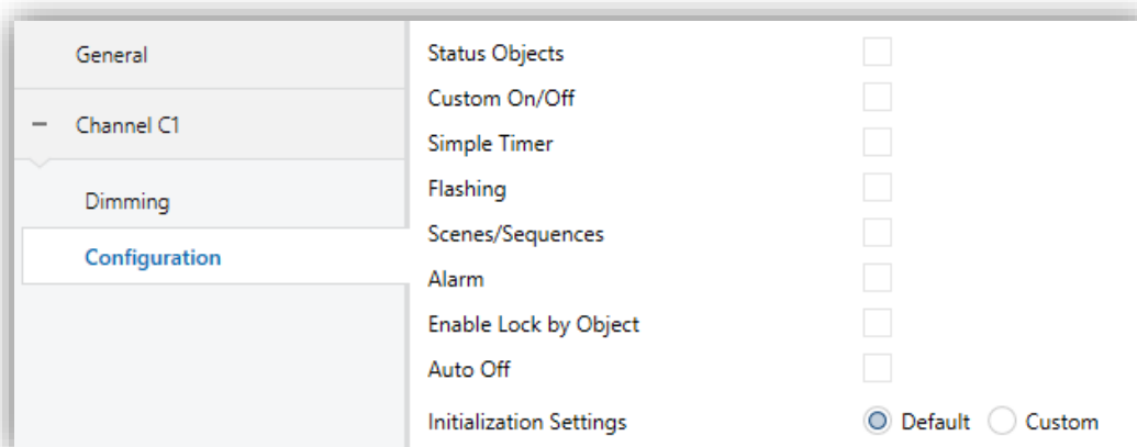
Figure 11 Configuration.
