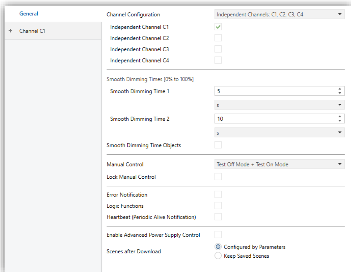
Figure 5 General - Configuration.
