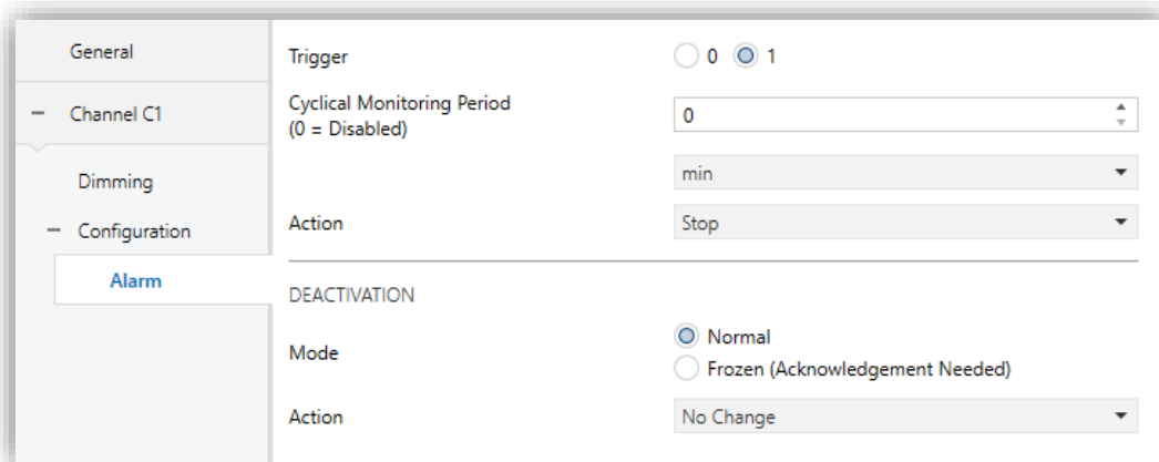
Figure 20 Alarm.
