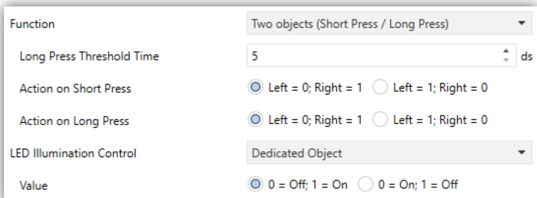
Figure 30 Pair Buttons - Two Objects (Short Press / Long Press).
