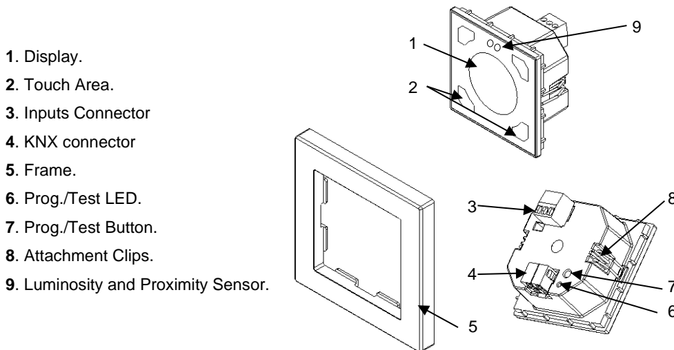
Figure 1. Schematic diagram.
