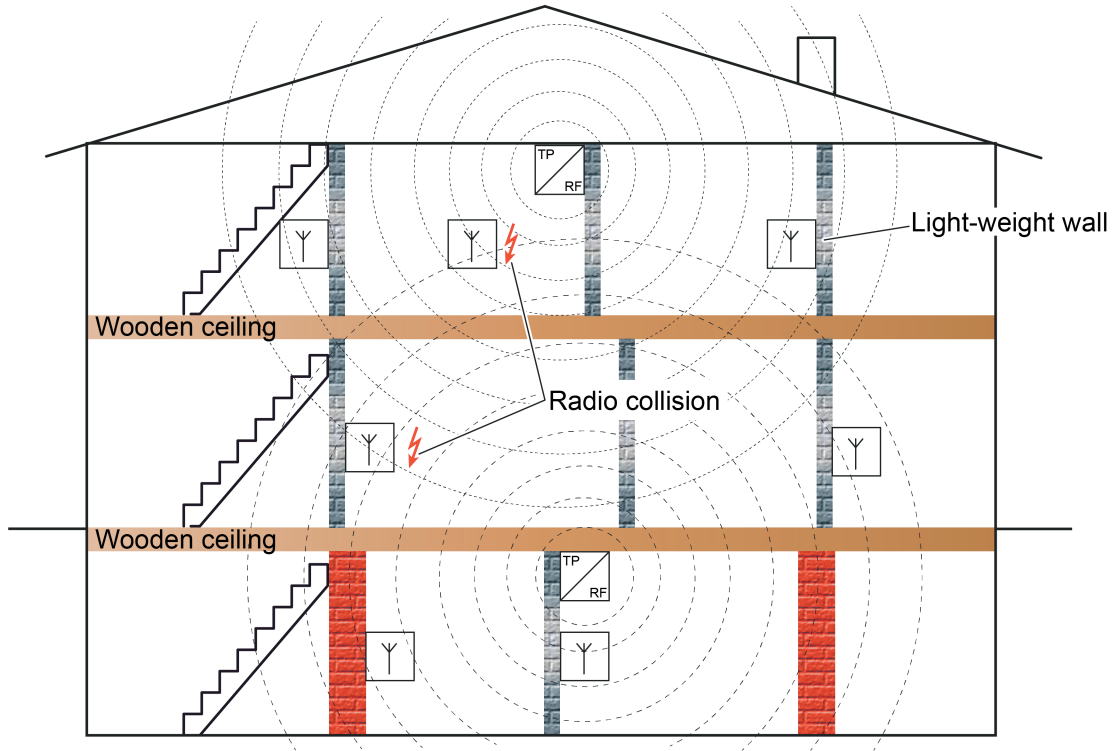
Figure 24: Building structure with two KNX RF lines, disadvantageous influence (example)
