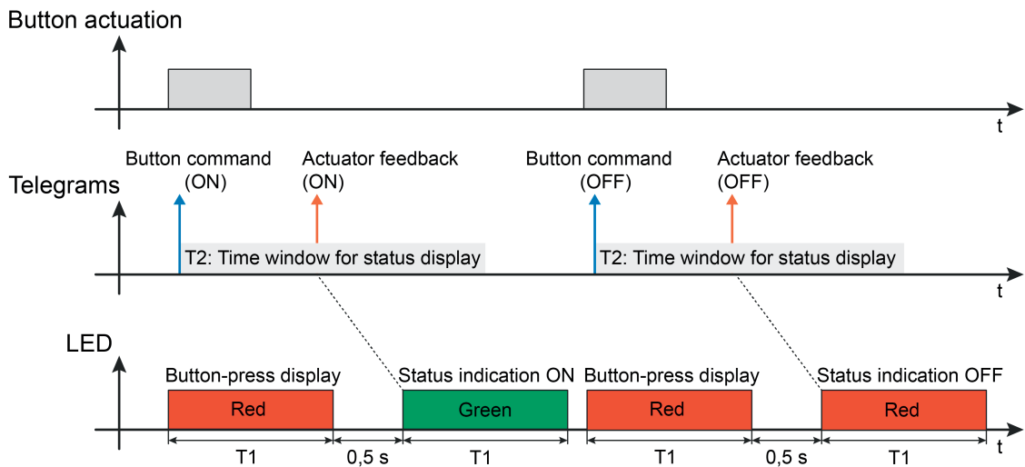
Figure 4: Example of a two-level actuation and status display with double status Status display state "ON" and "OFF" through green and red LED
