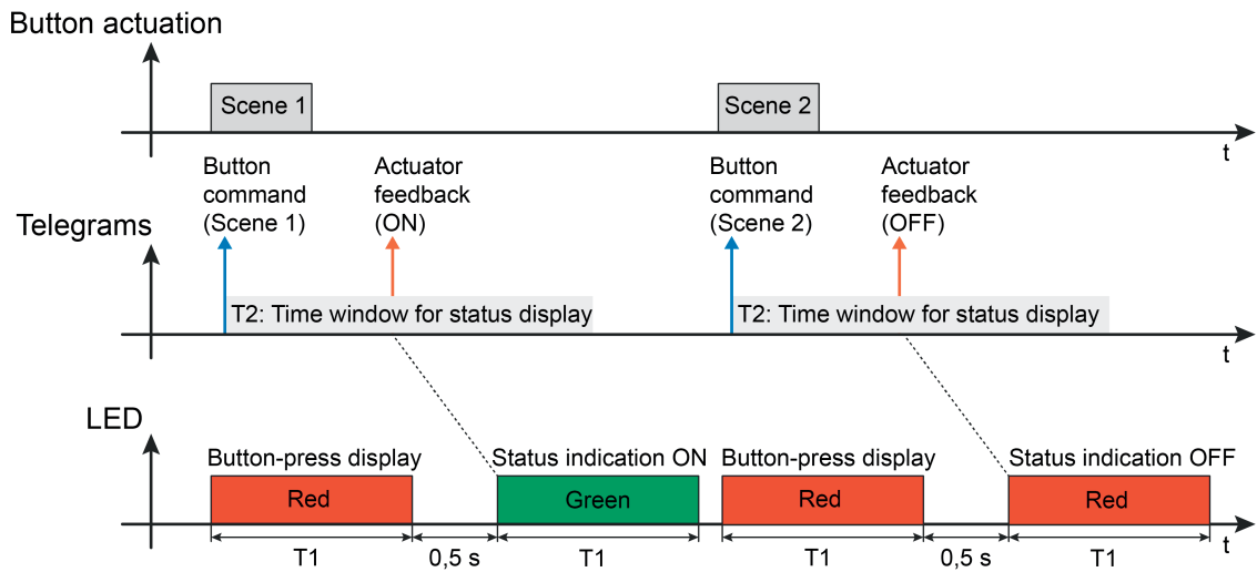
Figure 19: Example of a status display with the operating function "Scene extension" Scene extension without storage function (with double status ON and OFF)
