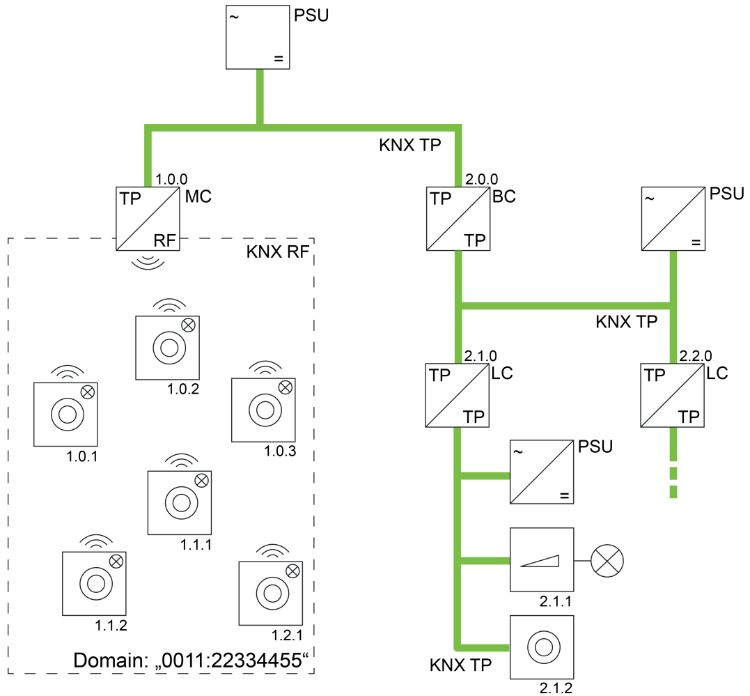
Figure 29: Example of a possible KNX topology with RF and TP lines Media coupler as backbone coupler
