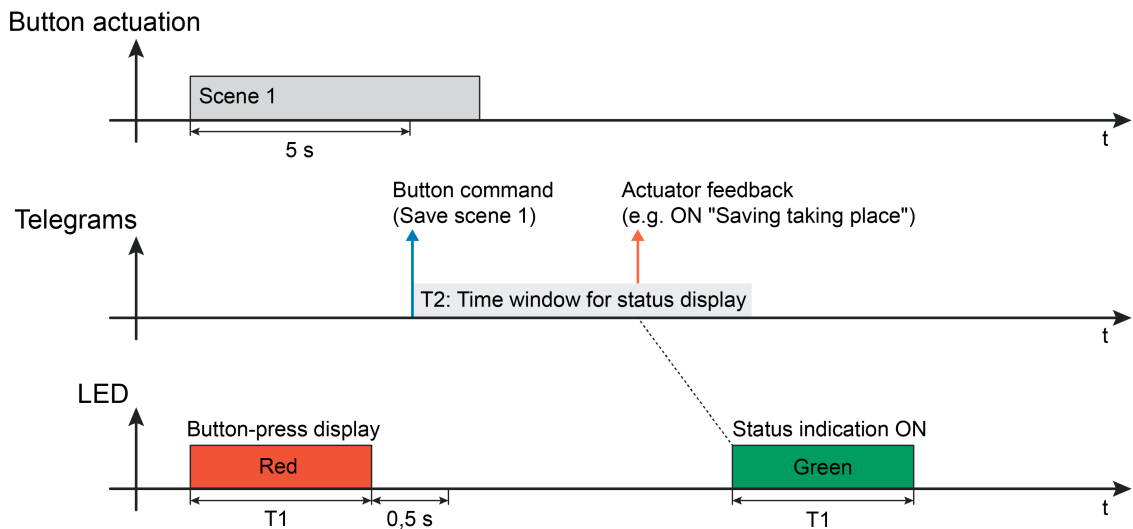
Figure 20: Example of a status display with the operating function "Scene extension" Scene extension with memory function and status display (with single status ON)
