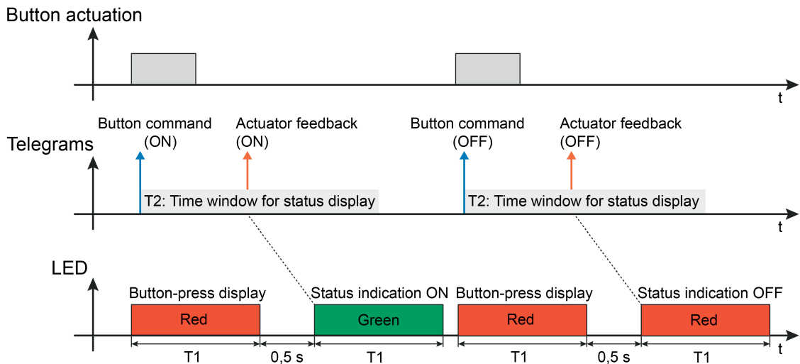
Figure 11: Example of a status display with the operating function "Switching" with double status (ON and OFF) Telegram on pressing the button
