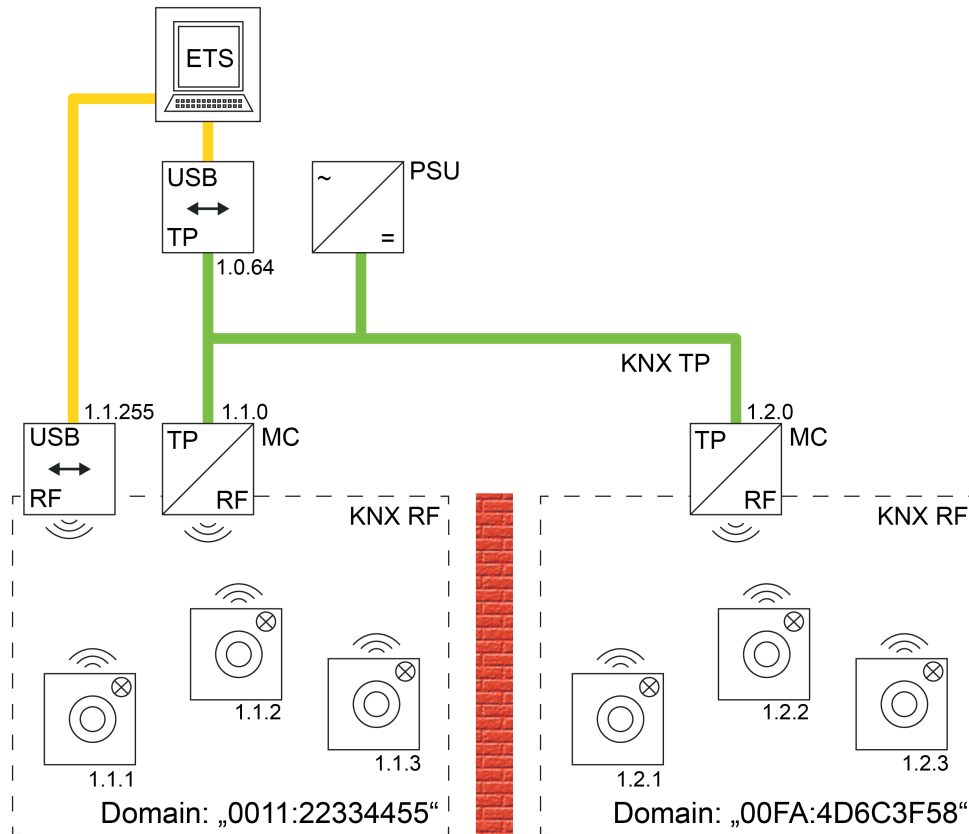
Figure 30: Example of a possible KNX topology with two RF lines and coupling via a TP main line (example)
