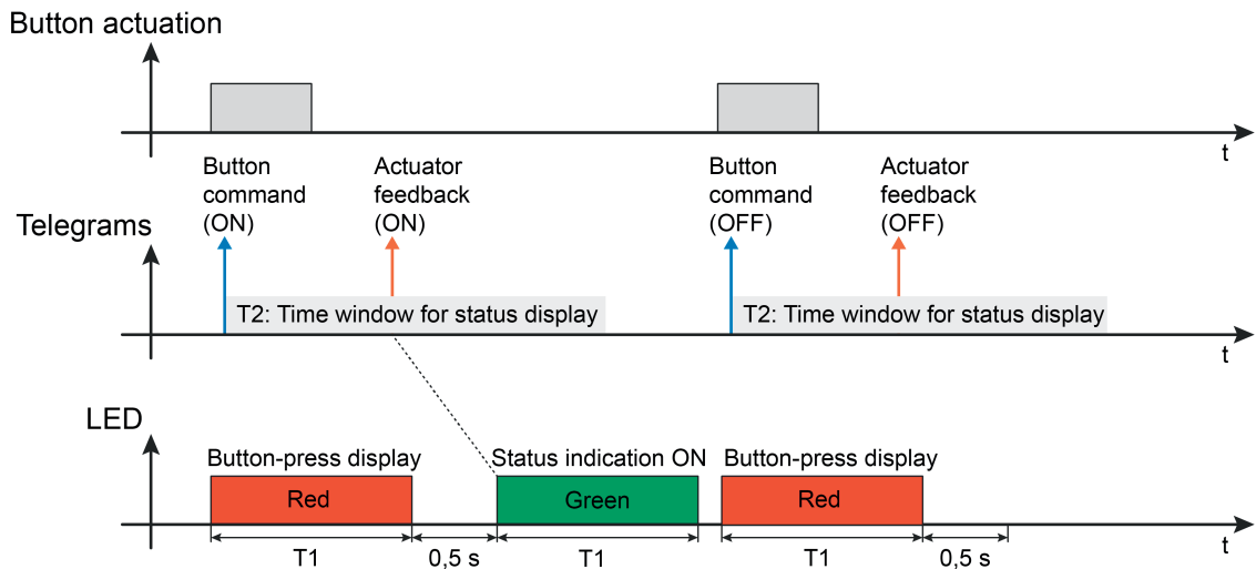
Figure 3: Example of a two-level actuation and status display with single status Status display state "ON" through green LED
