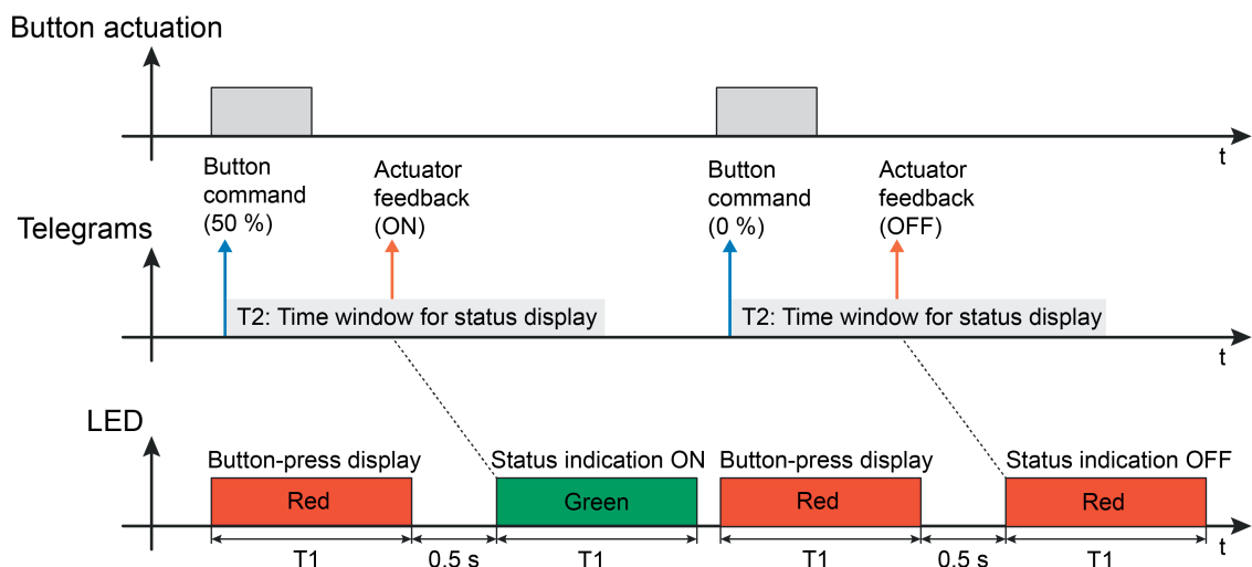
Figure 18: Example of a status display with the operating function "Value transmitter 1-byte" with double status (ON and OFF) Telegram on pressing the button
