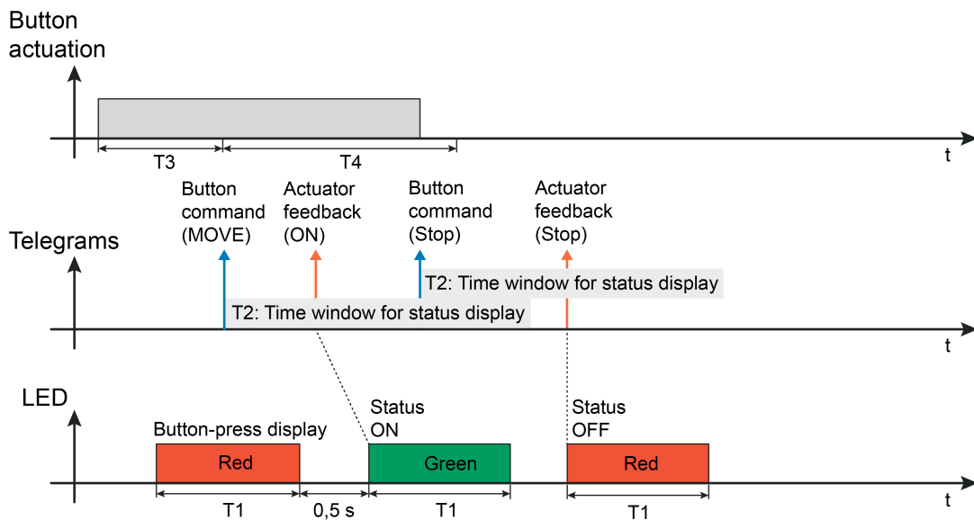
Figure 17: Example of a status display with the operating function "Venetian blind" with a long button-press
