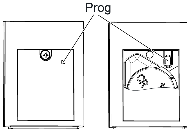
Figure 2: Programming button in battery compartment
