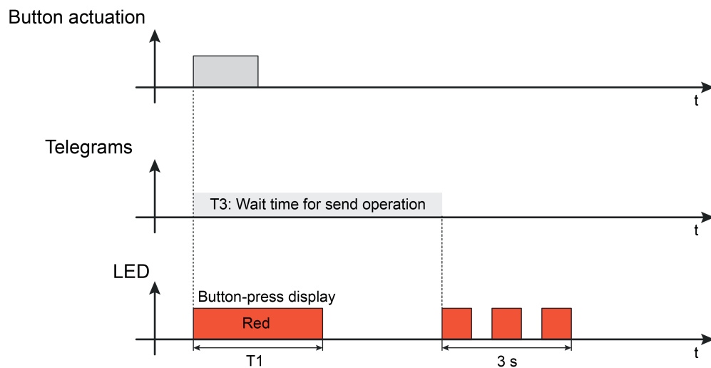
Figure 10: LED display in the case of a transmission error
