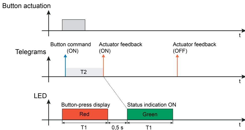
Figure 8: Example of a two-level actuation and status display with double status Reception of two actuator status messages in time window not permitted
