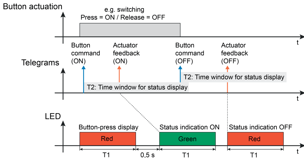
Figure 5: Example of a two-level actuation and status display with double status New time window for status display through multiple operating telegrams
