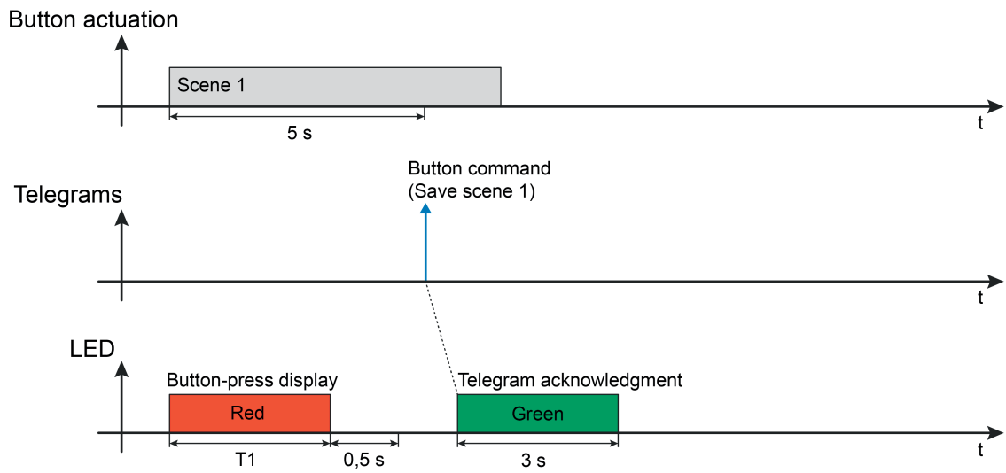
Figure 21: Example of an LED display with the operating function "Scene extension" Scene extension with memory function and telegram acknowledgement
