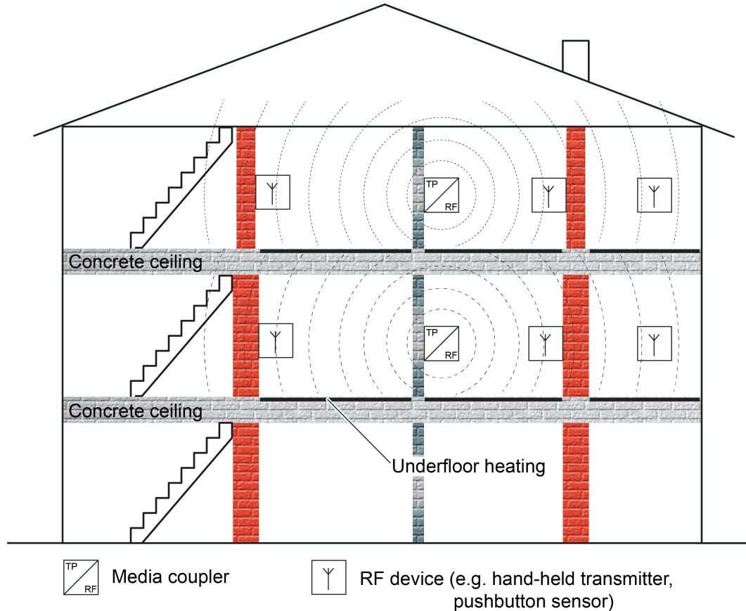
Figure 26: Building structure with two KNX RF lines, which do not influence each other negatively due to the building consistency (example)
