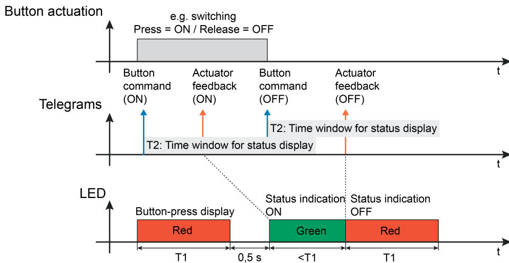
Figure 6: Example of a two-level actuation and status display with double status Interruption of the first status display through the actuator status in the new time window
