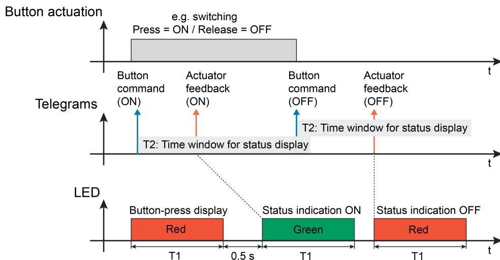
Figure 12: Example of a status display with the operating function "Switching" with double status (ON and OFF) Telegram on pressing and releasing the button
