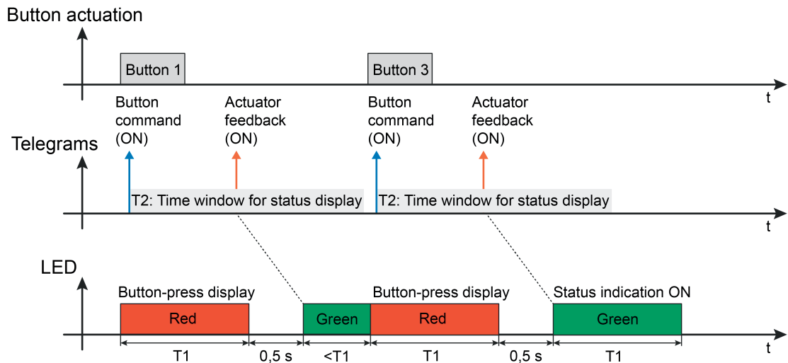
Figure 9: Example of a two-level actuation and status display Interruption of the display function through new button actuation
