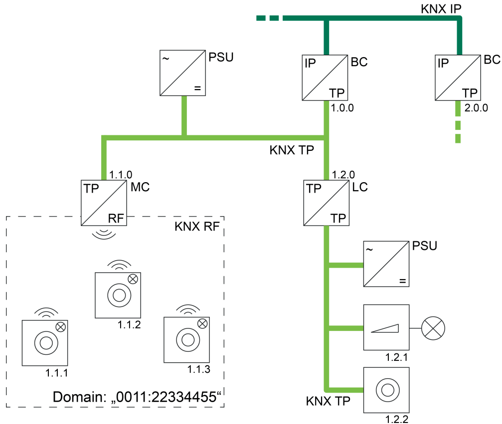
Figure 28: Example of a possible KNX topology with RF, TP and IP lines Media coupler as line coupler
