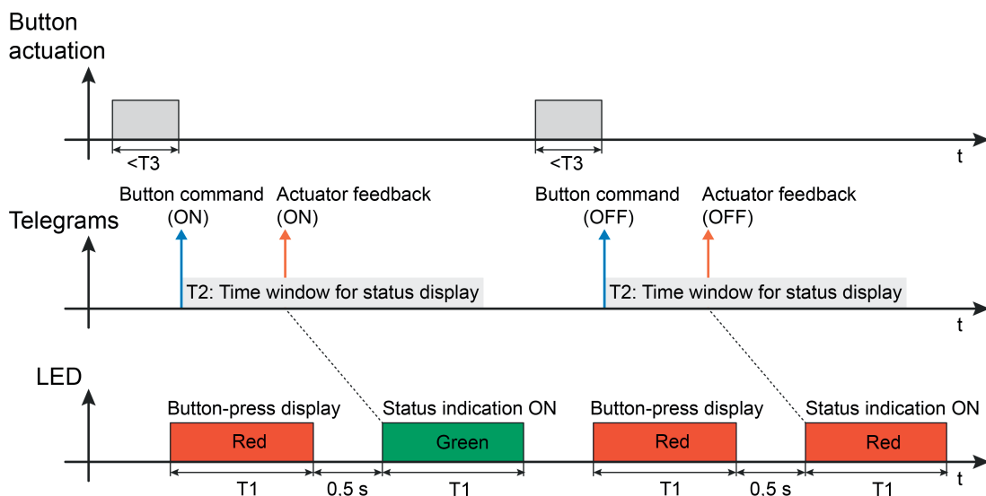
Figure 13: Example of a status display with the operating function "Dimming" with a short button-press (with double status ON and OFF)
