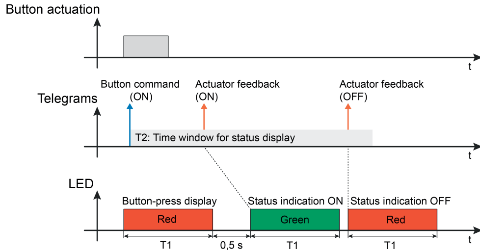
Figure 7: Example of a two-level actuation and status display with double status Reception of two actuator status messages in time window permitted
