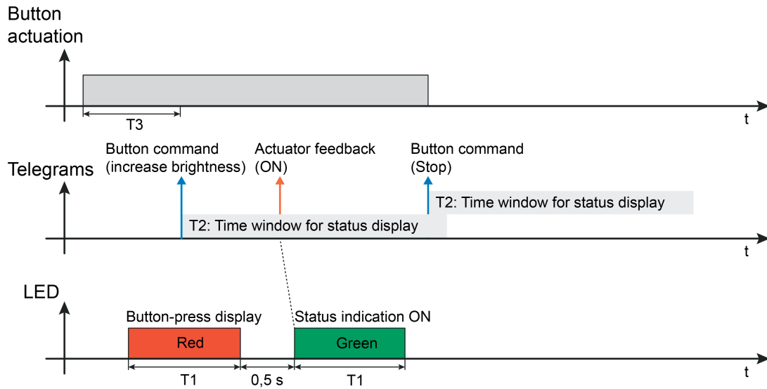
Figure 14: Example of a status display with the operating function "Dimming" with a long button-press
