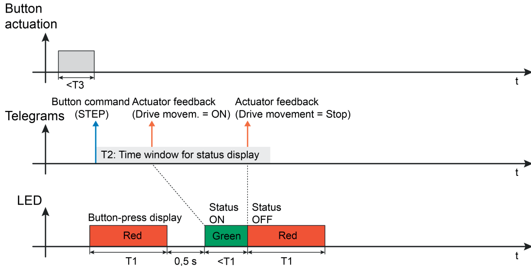
Figure 16: Example of a status display with the operating function "Venetian blind" with a short button-press (with double status ON and OFF)
