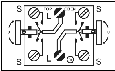
Contact assignments
