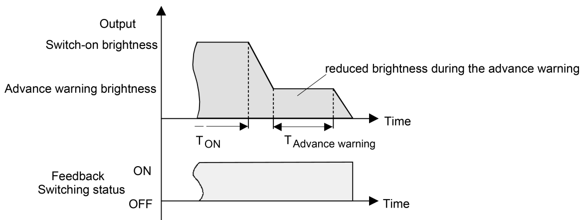
Image 21: The pre-warning function of the staircase function with soft OFF function (as an example with minimum brightness = 0%)
