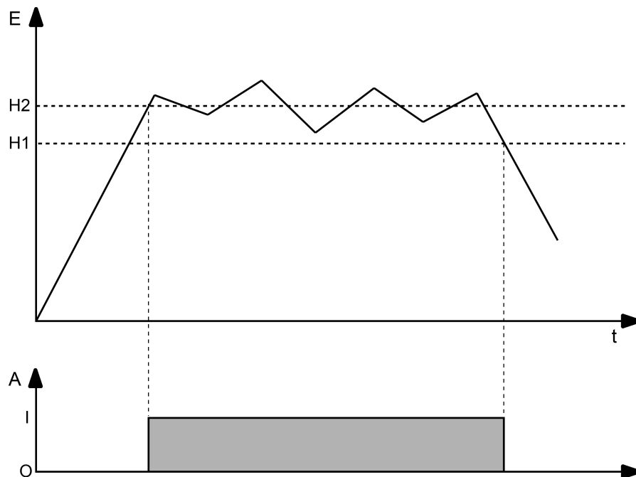
Image 32: Example of a hysteresis evaluation by upper and lower threshold value.
