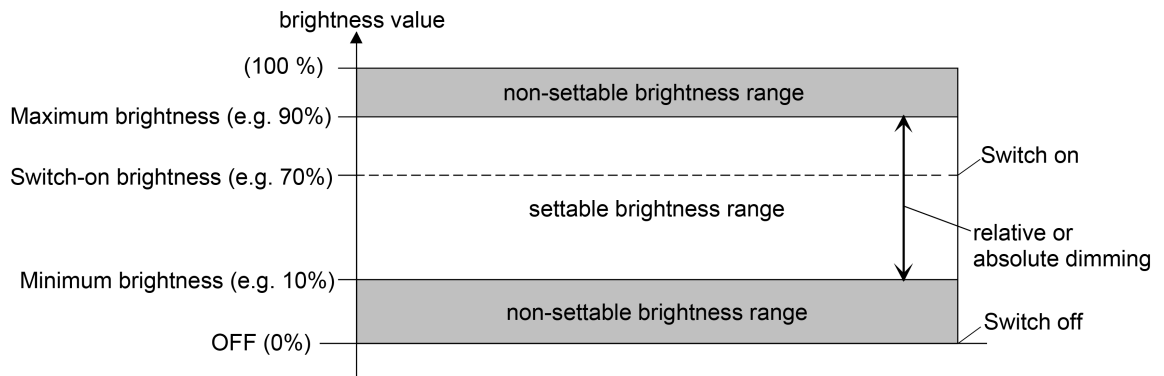
Image 12: Example of a brightness range with minimum brightness
