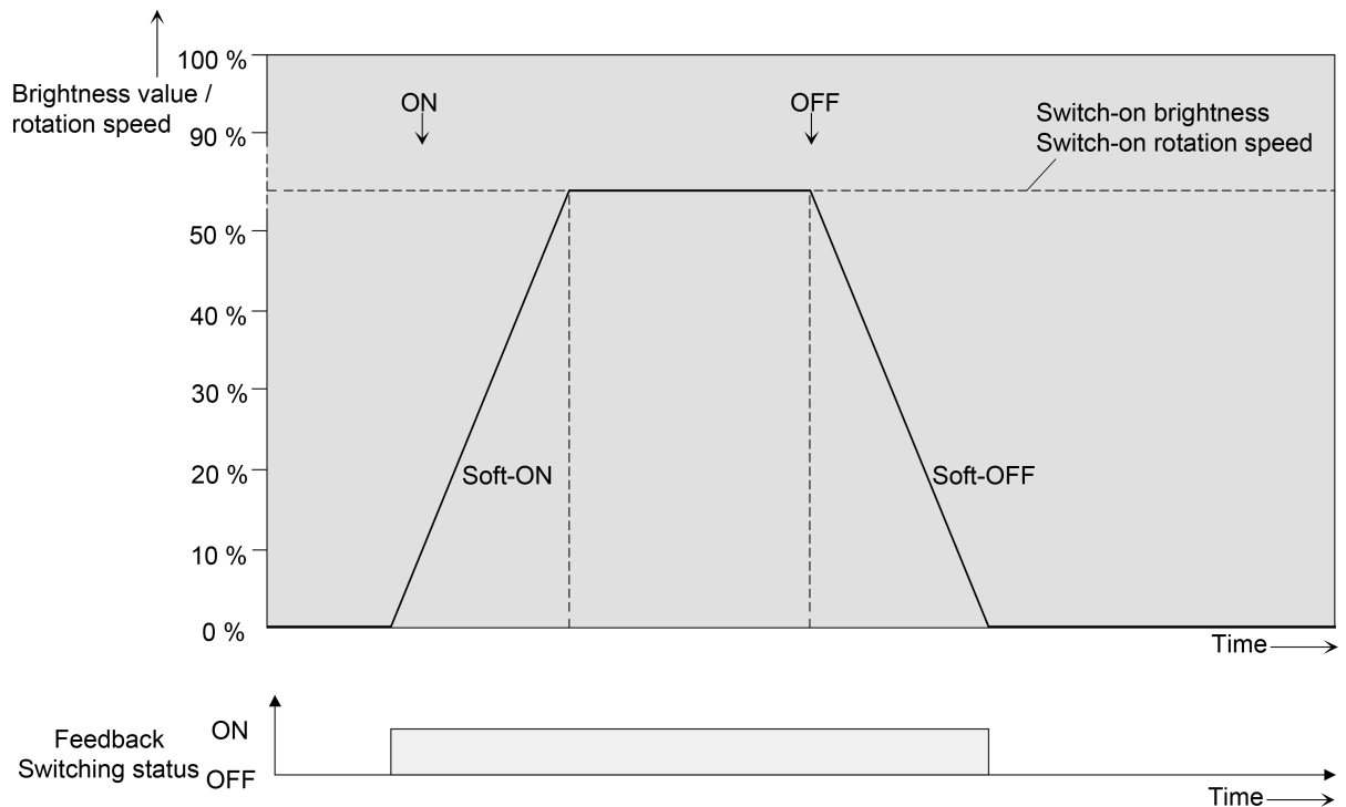
Image 14: Dimming behaviour of the soft ON/OFF functions (as an example)
