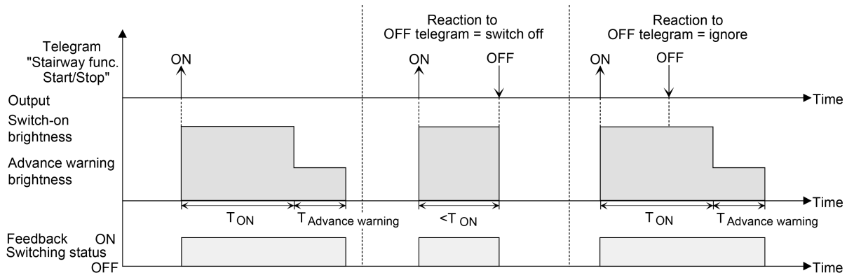
Image 18: Switch-off behaviour of the staircase function without soft functions
