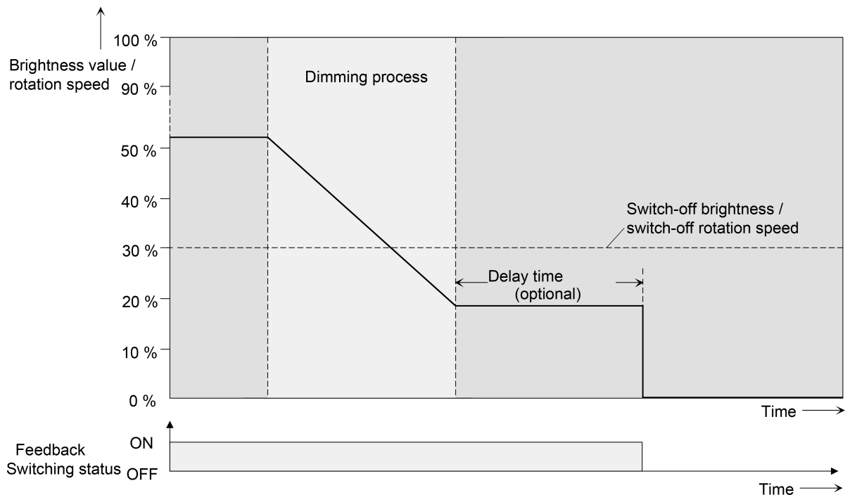
Image 15: Dimming and switching behaviour of the automatic switch-off function
