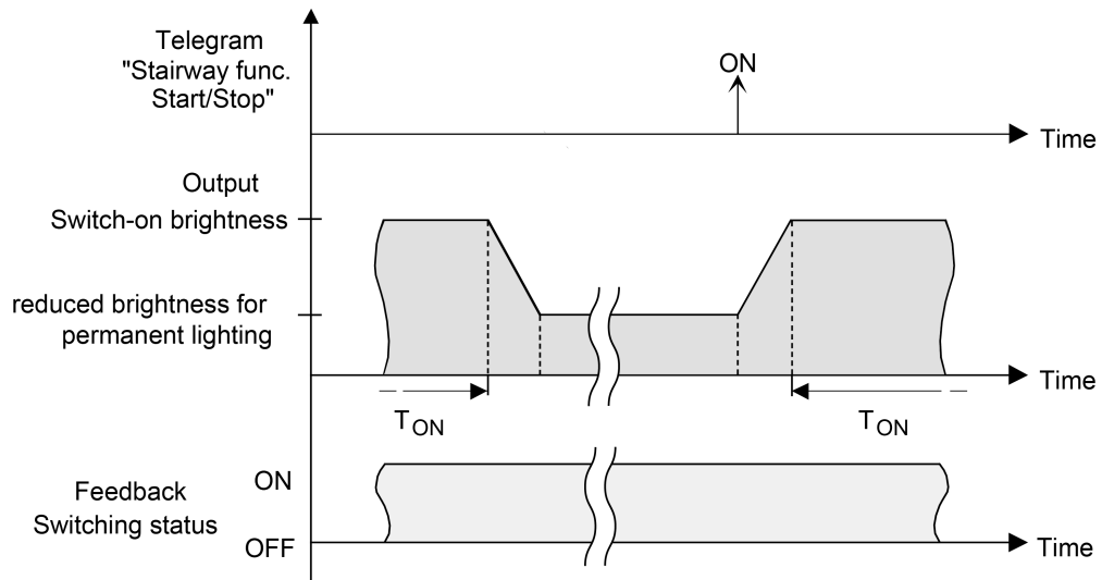
Image 23: The continuous lighting of the staircase function with soft OFF functions
