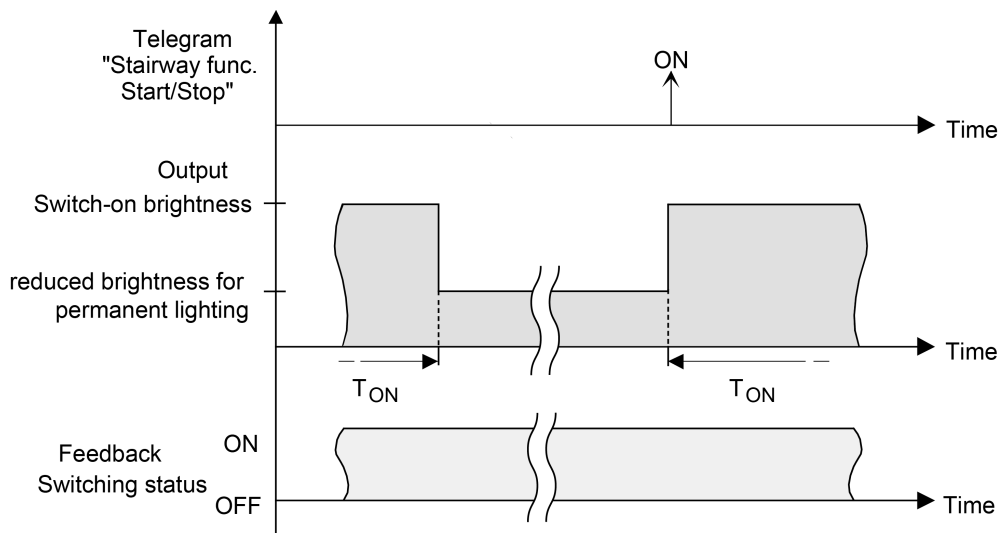
Image 22: The continuous lighting of the staircase function without soft functions
