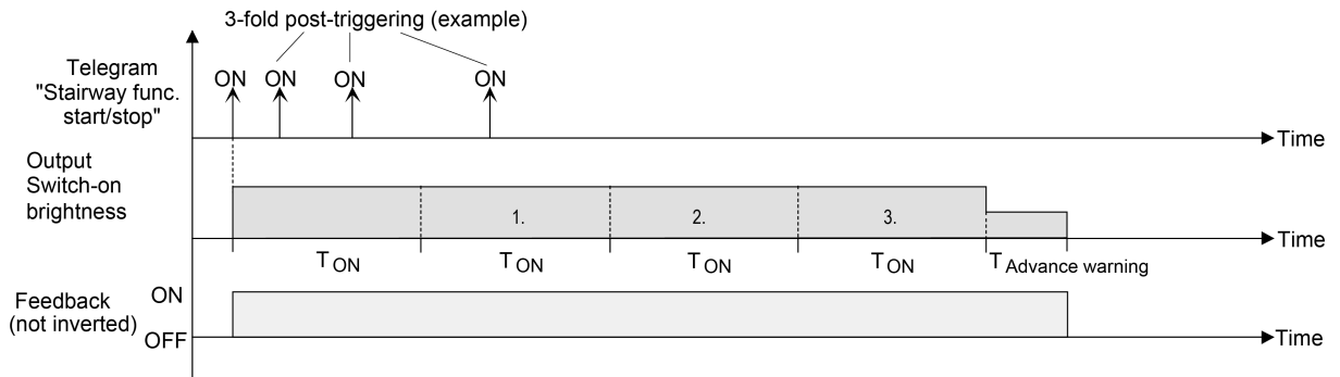
Image 24: Time extension of the staircase function
