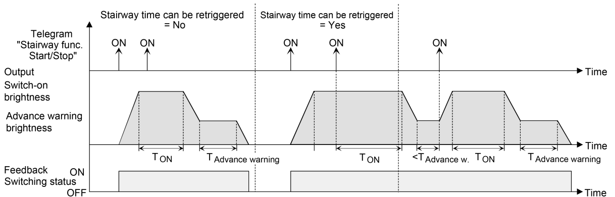
Image 17: Switch-on behaviour of the staircase function with soft functions (as an example with minimum brightness = 0 %)
