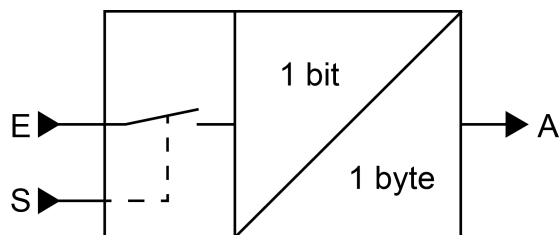
Image 27: converter (1 bit -> 1 byte)
