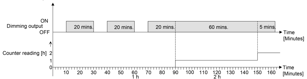
Image 26: Function of the operating hours counter (using the example of counted hours)
