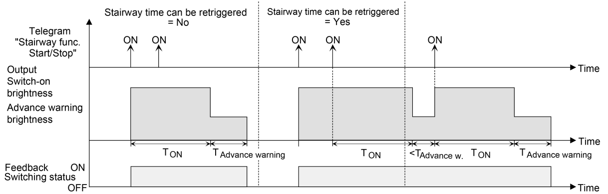
Image 16: Switch-on behaviour of the staircase function without soft functions
