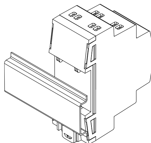
Figure 3: Mounting ShutterBOX Drive 2CH on DIN rail
