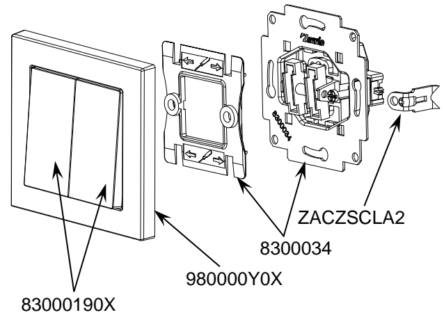
Figure 1. Double two-way rocker switch
